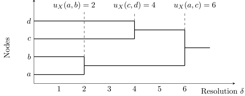
Figure 2.2: Equivalence of dendrograms and ultrmetrics. Given a dendrogram D_X define the function u_X(x, x') := \min \{ \delta \geq 0 \mid x \sim_{D_X(\delta)} x' \} . This function is an ultrmetric because it satisfies the identity property, the strong triangle inequality (2.12) and is symmetric.
