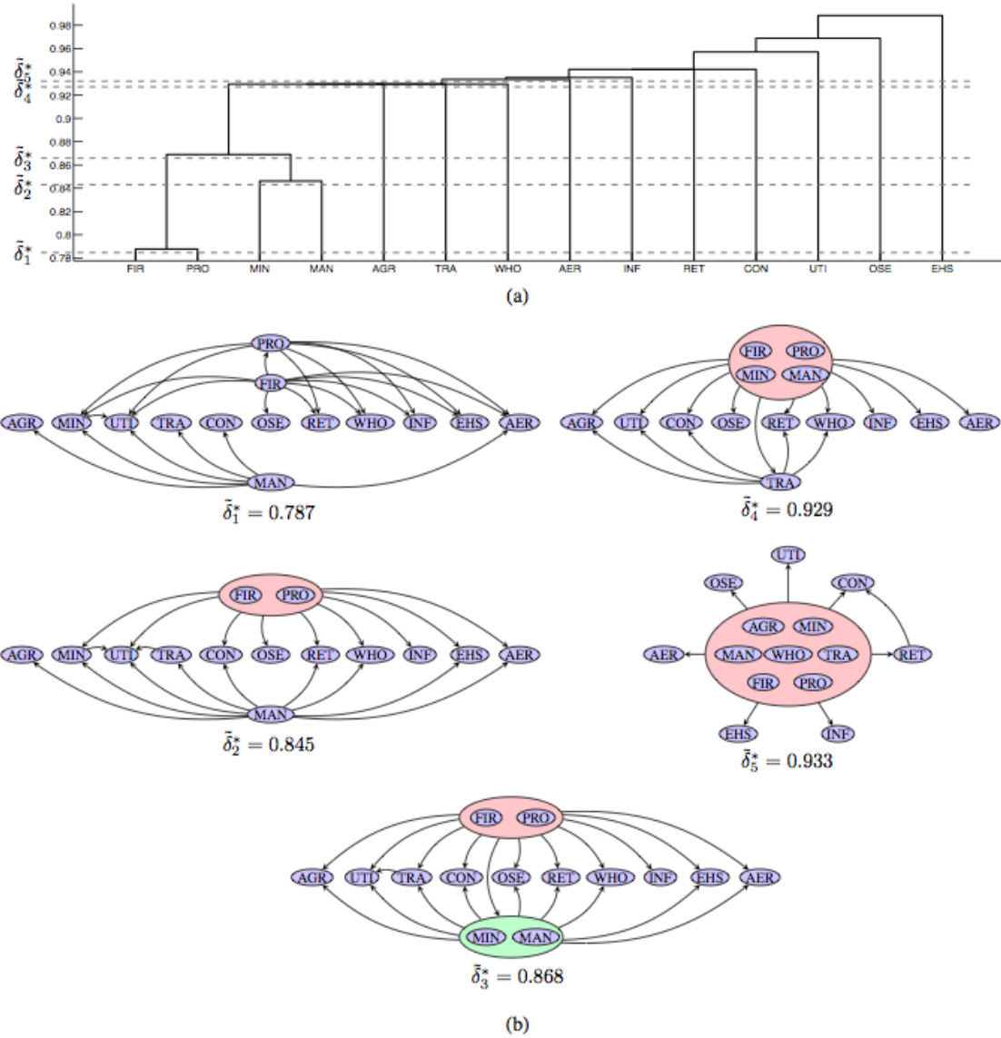
Figure 6.10: (a) Dendrogram component D_C^* of the quasi-dendrogram \tilde{D}_C^* = (D_C^*, E_C^*) . Output of the directed single linkage quasi-clustering method \tilde{\mathcal{H}}^* when applied to the network N_C . (b) Quasi-partitions. Given by the specification of the quasi-dendrogram \tilde{D}_C^* at a particular resolution \tilde{D}_C^*(\tilde{\delta}_k^*) for k = 1, \dots, 5 .
