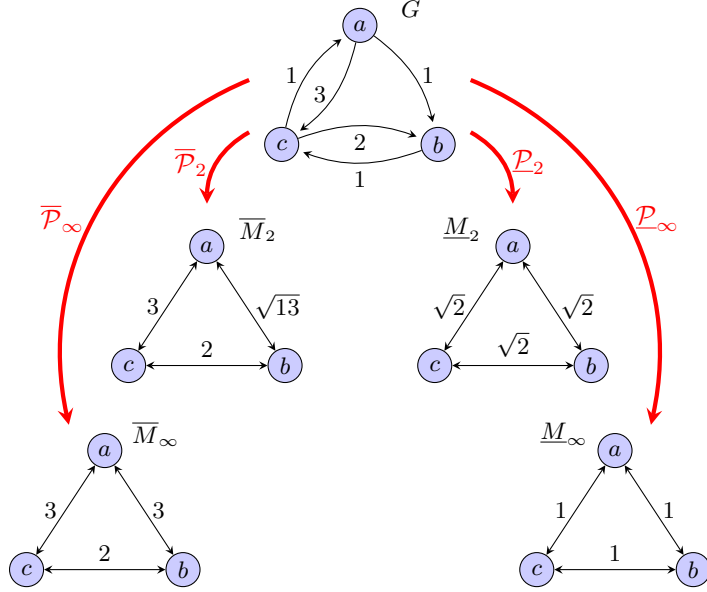
Figure 10.2: The q -metric spaces obtained by applying \overline{\mathcal{P}}_q and \mathcal{P}_q to network G for q = 2 and q = \infty .
