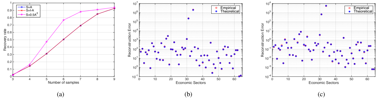
Fig. 1: (a) Recovery rate of bandlimited signals with unknown support as a function of the number of samples. (b) Empirical and theoretical reconstruction errors for different sampling nodes when white noise is added to the observed signal. (c) Empirical and theoretical reconstruction errors when white noise is added directly to the signal \mathbf{x}_4 .
